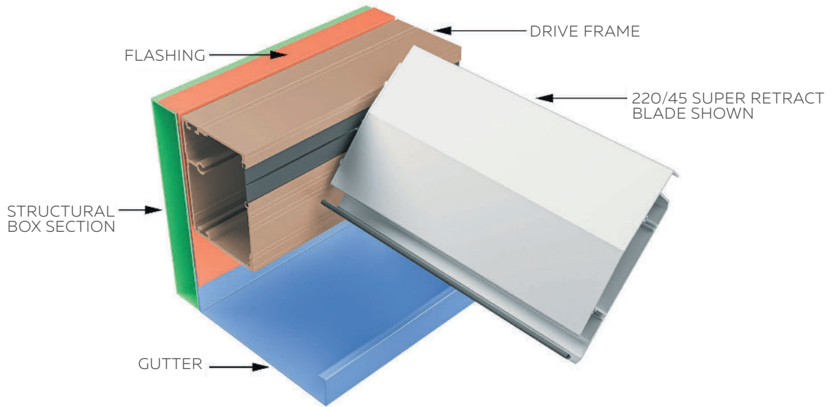
CROSS SECTION SHOWING DRIVE FRAME, BLADE, GUTTER & FLASHING WITHIN 300X50 BOX SECTION FRAME
